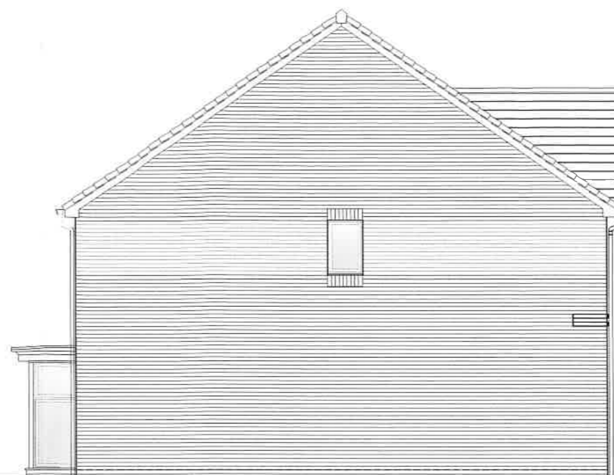
Left Elevation
